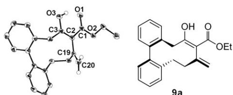
Figure 1. ORTEP drawing of the ten-membered ring product 9a (50% probability for thermal ellipsoids). Hydrogen atoms except for those on O3 and C20 are omitted for clarity. Selected bond lengths [Å]: C(1)–C(2) 1.4626(17), C(2)–C(3) 1.3587(18), C(2)–C(19) 1.4959(15), C(19)–C(20) 1.3208(18).
