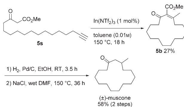
Scheme 2. Synthesis of ( \pm )-muscone through the fifteen-membered ring product 5b . DMF = N,N -dimethylformamide.
